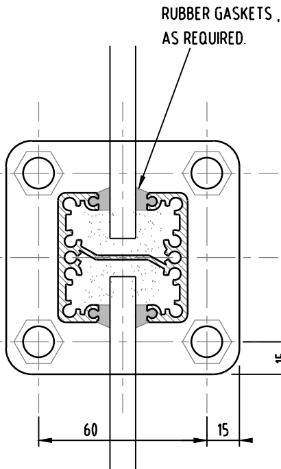
APR 'BSQP' BASEPLATE ( SCALE 1:2 )
